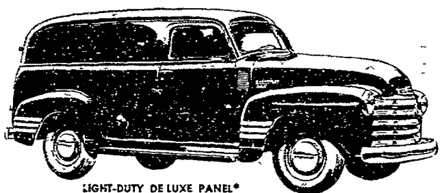
LIGHT-DUTY DE LUXE PANEL* Model 3105—116 inch wheelbase, Maximum G.V.W. 4,600 lb. Also available in Medium-Duty model 3805—137 inch wheelbase, Maximum G.V.W. 6,700 lb.
