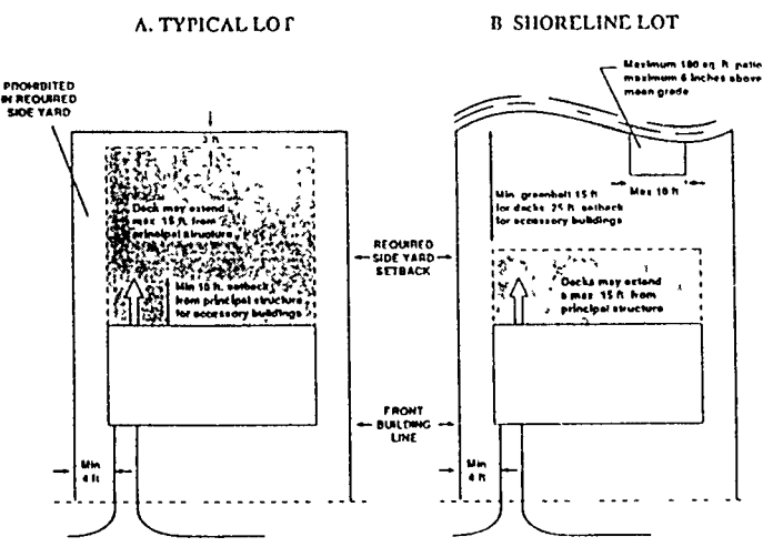
FIGURE 18.11 ACCESSORY BUILDINGS AND STRUCTURES LOCATION STANDARDS
