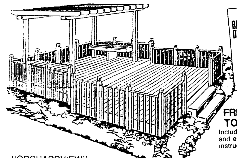
"ORCHARDVIEW" 2 - 10'x14' BI-LEVEL DECK
