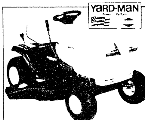
13.5 HP/38" LAWN TRACTOR 13.5 HP Briggs & Stratton diamond plus engine with yard man hydrostatic transmission. Heavy duty tractor box frame. 18 x 8.5 inch tires.
