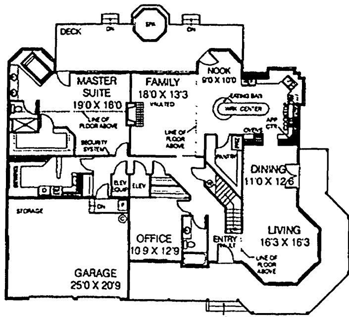
FIRST FLOOR PLAN Copley News Service
