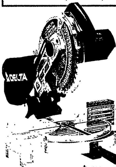
10" Compound Power Miter Saw • 13 amp; 120 volt; 5,200 rpm • Easy-to-read bevel scale #21384
