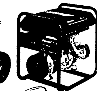
10 HP, 5,250 Watt Generator • 7 gallon extended run gas tank • Cast iron cylinder sleeve • Tecumseh engine #34386
