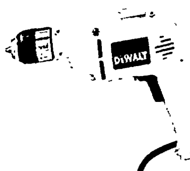
3/8 inch Heavy-Duty VSR Drill • 5.4 amp; 0-2,500 rpm • Includes case • Keyless chuck • All ball bearing construction #19808
