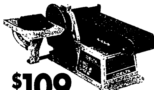
4" Belt/6" Disc Sander • 1/2 HP; 3,100 rpm disc speed • 2,000 sfm belt speed #98646
